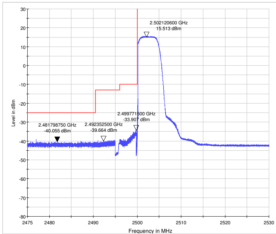
LTE Band 7 QPSK 5MHz CH-Low, RB 25
