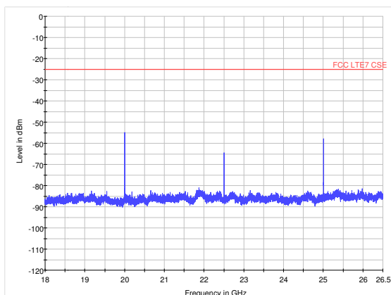
LTE Band 7 5MHz CH-Low 18GHz~26.5GHz
