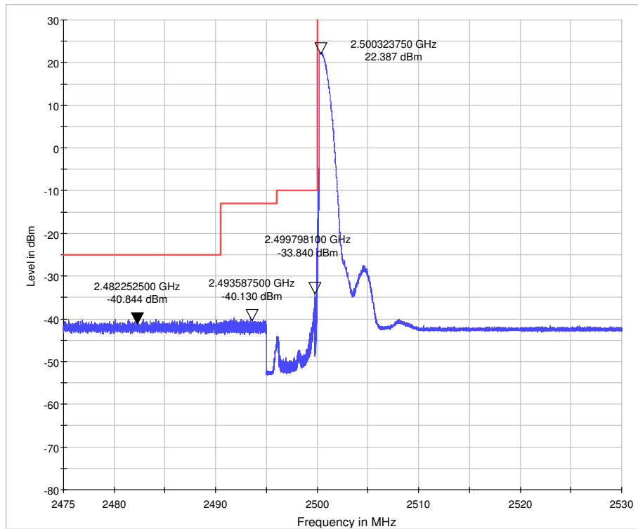
LTE Band 7 QPSK 5MHz CH-Low, RB 25
