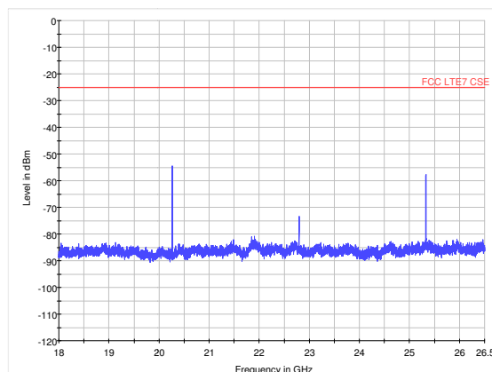
LTE Band 7 5MHz CH-Middle 18GHz~26.5GHz
