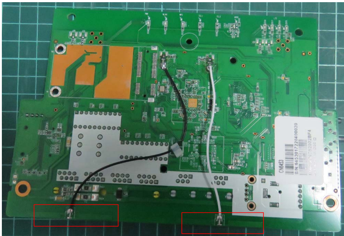
WiFi Antenna
