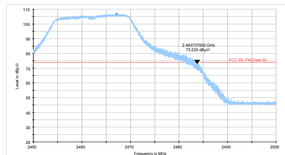
802.11g-Channel 11: Peak
