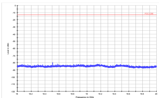
LTE Band 2 15MHz CH-Low 18GHz~20GHz
