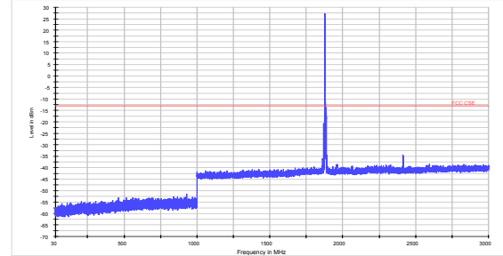
LTE Band 2 5MHz CH-Middle 30MHz~3GHz
