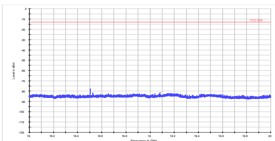
LTE Band 2 5MHz CH-Low 18GHz~20GHz
