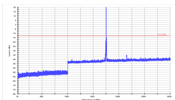
LTE Band 4 5MHz CH-High 30MHz~3GHz
