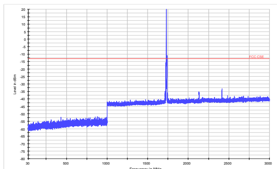
LTE Band 4 5MHz CH-High 30MHz~3GHz
