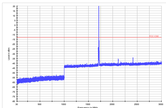
LTE Band 4 5MHz CH-Middle 30MHz~3GHz
