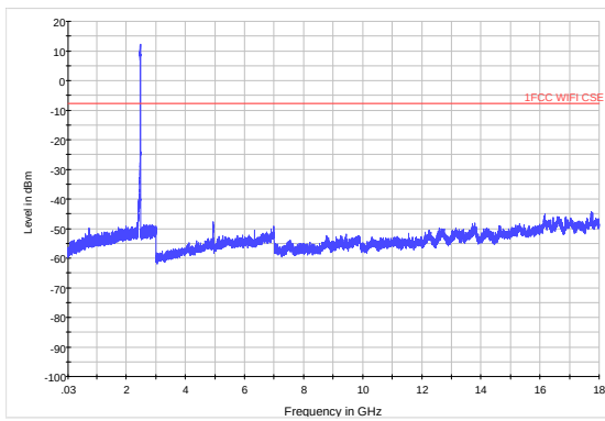
802.11g CH13 30MHz to 18GHz
