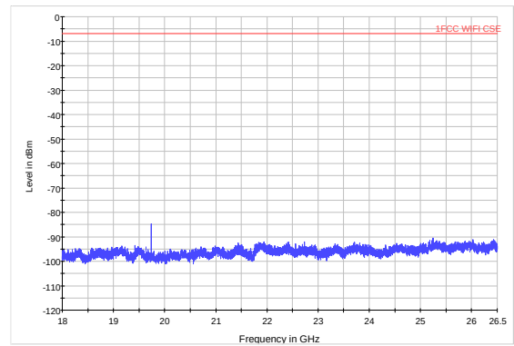
802.11n (HT20) CH12 18GHz to 26.5GHz
