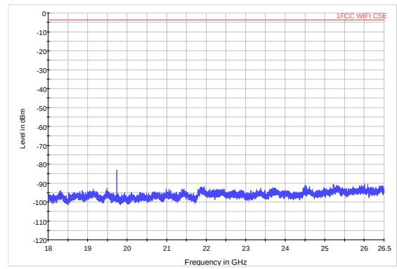
802.11b CH12 18GHz to 26.5GHz
