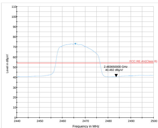
802.11n HT20-Channel 12: Average
