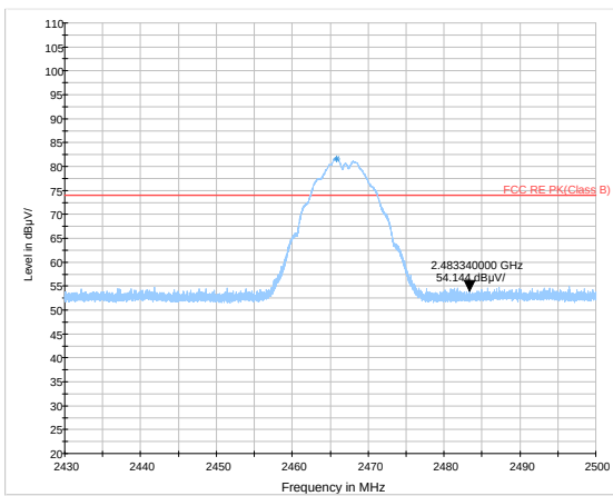
802.11b-Channel 12: Peak
