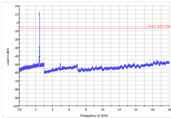
802.11n (HT20) CH12 30MHz to 18GHz
