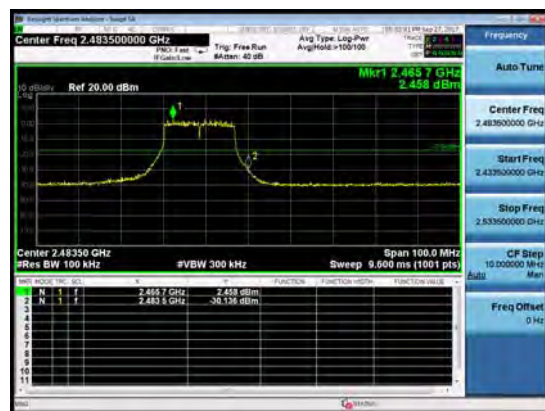
802.11g, Channel No.: 13
