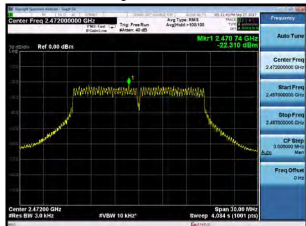
802.11g, Channel No.: 13
