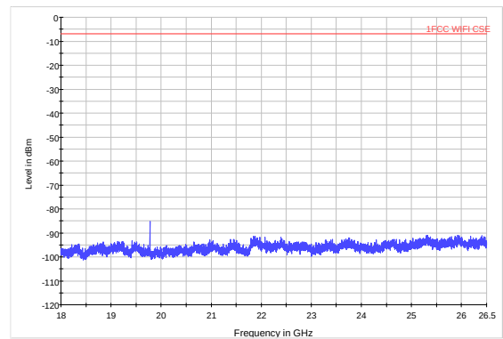
802.11n (HT20) CH13 18GHz to 26.5GHz
