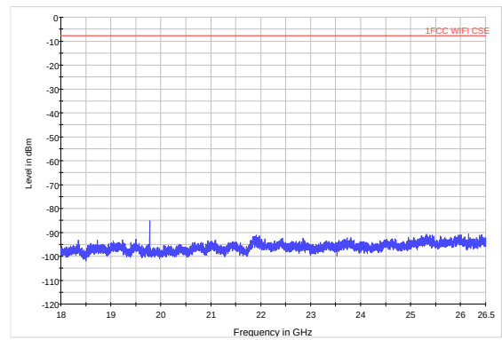
802.11g CH13 18GHz to 26.5GHz
