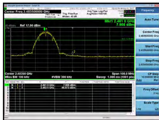
802.11b, Channel No.: 13
