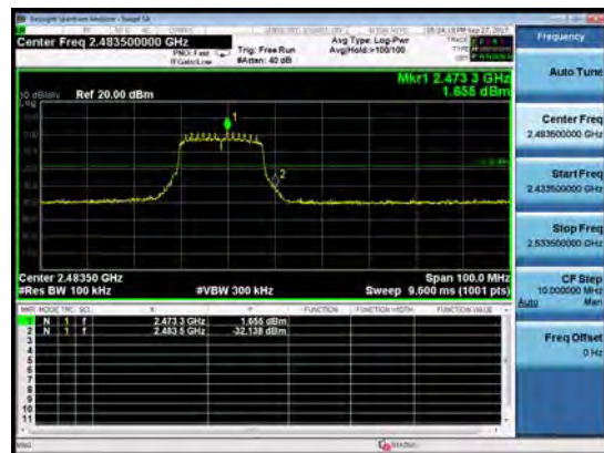
802.11n(HT20), Channel No.: 13
