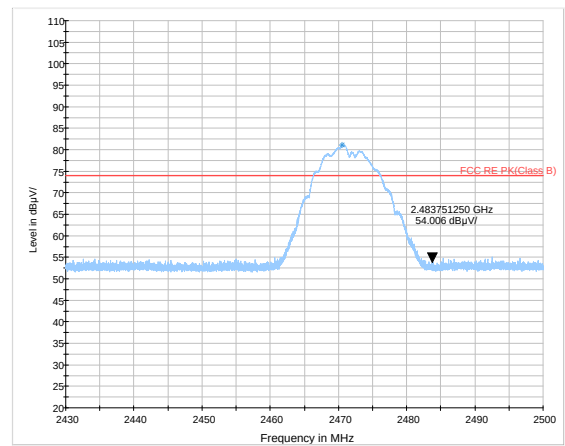
802.11b-Channel 13: Peak
