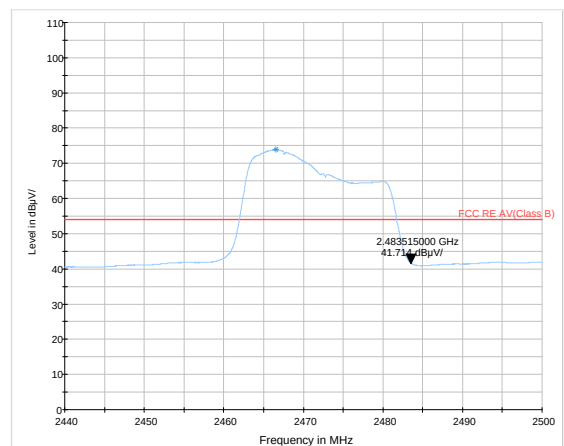
802.11n HT20-Channel 13: Average
