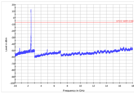
802.11g CH12 30MHz to 18GHz
