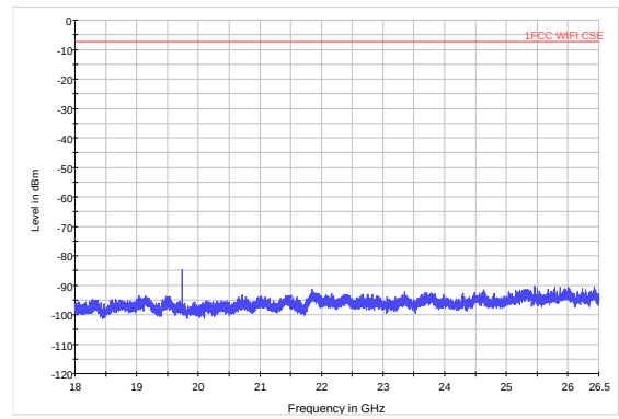
802.11g CH12 18GHz to 26.5GHz
