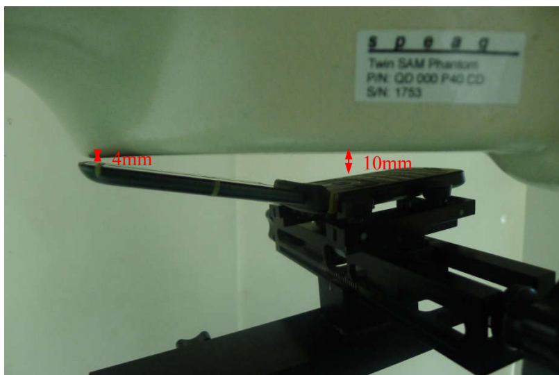
GSM1900/WCDMA Band II/LTE Band 2 SAR in mouth area(Flip Open)
