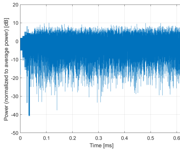
Time Domain
