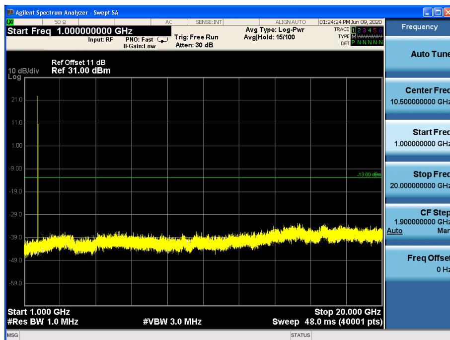
Channel 1412, 1GHz~20GHz
