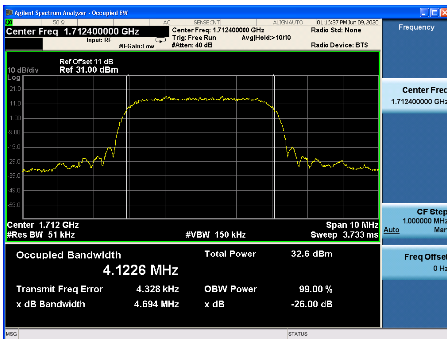
Channel 1312
