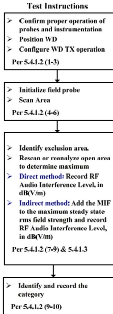
Test flowchart Per ANSI-C63.19
