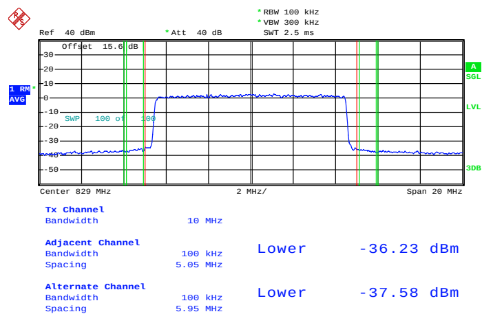
Lower Band Edge Plot for QPSK-RB Size 50, RB Offset 0
