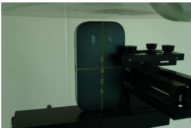
Left Side of the DUT with Phantom 10 mm Gap
