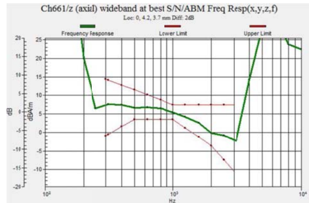
Fig 9.2 GSM1900 Ch661
