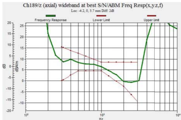
Fig 9.1 GSM850 Ch189
