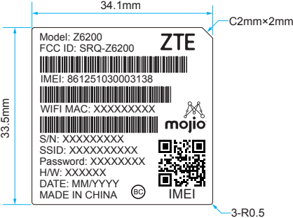
Size: 34.1*33.5*0.15mm, 3-R0.5 Material code: 5646125300MT
