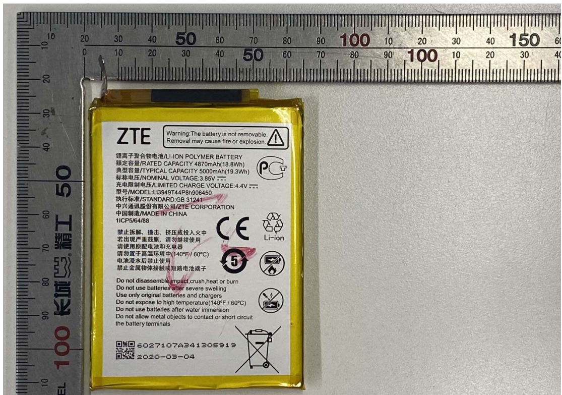
Battery View 1
