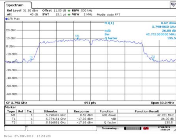
Test Mode: 802.11n HT40 5795MHz
