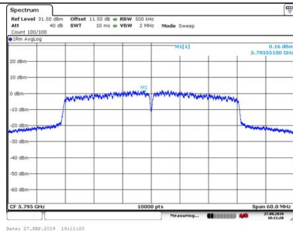
Test Mode: 802.11n HT40 Chain0
