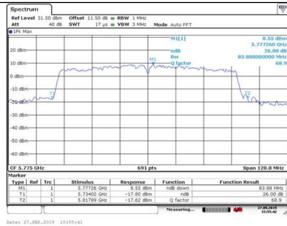
Test Mode: 802.11ac VHT80 5775MHz
