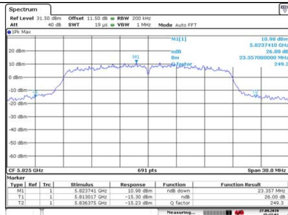
Test Mode: 802.11n HT20 5825MHz
