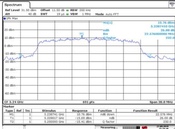
Test Mode: 802.11n HT20 5240MHz
