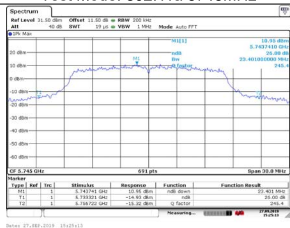
Test Mode: 802.11a 5745MHz
