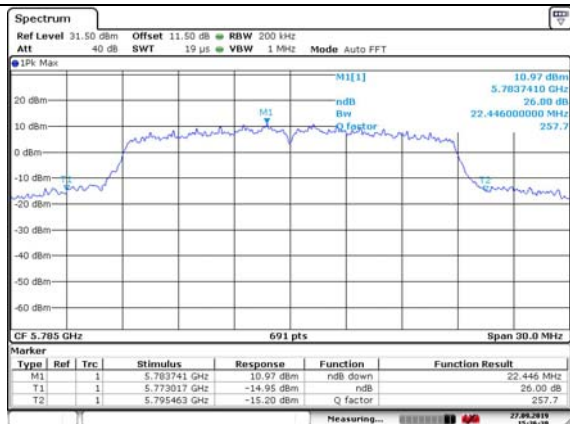
Test Mode: 802.11n HT20 5785MHz
