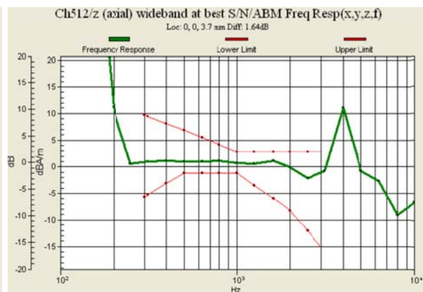
Fig 7.4 GSM1900 Ch512
