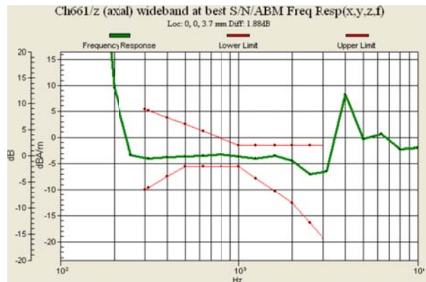
Fig 7.2 GSM1900 Ch661
