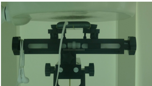
Back with Headset, Test Separation 1 cm
