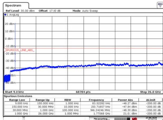
EN-DC_2A_n66 10MHz CH-High 9kHz~26GHz
