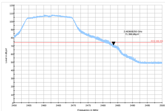
802.11g-Channel 11 Peak
