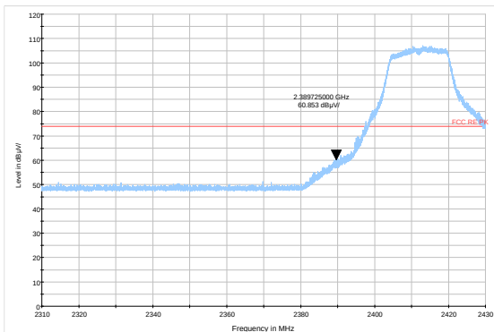
802.11g-Channel 1 Peak
