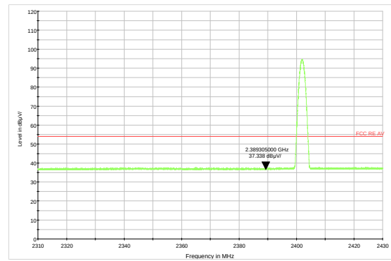
BLE-1M Channel 0 Average
