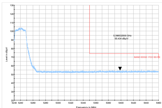
802.11a-Channel 48: Average
