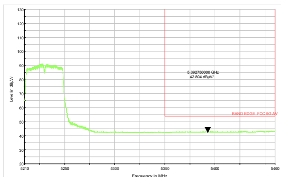
802.11ac VHT80- Channel 42: Average
