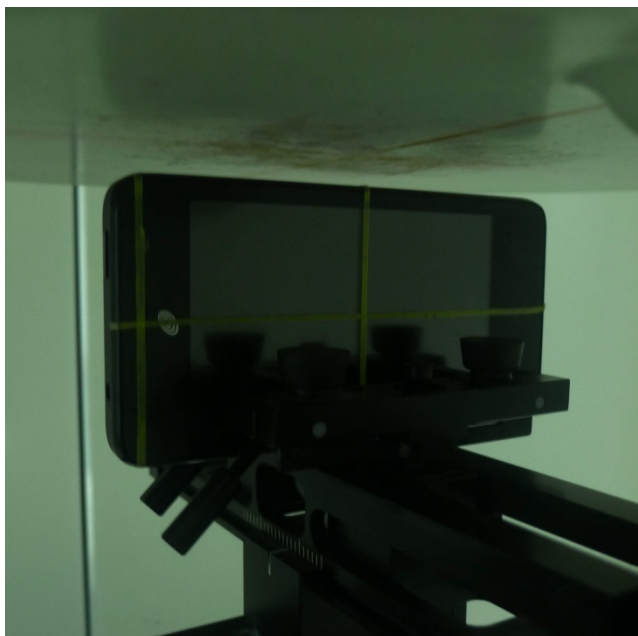
Right Side of the DUT with Phantom 1 cm Gap
