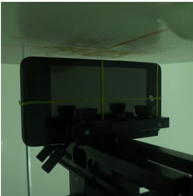
Left Side of the DUT with Phantom 1 cm Gap
