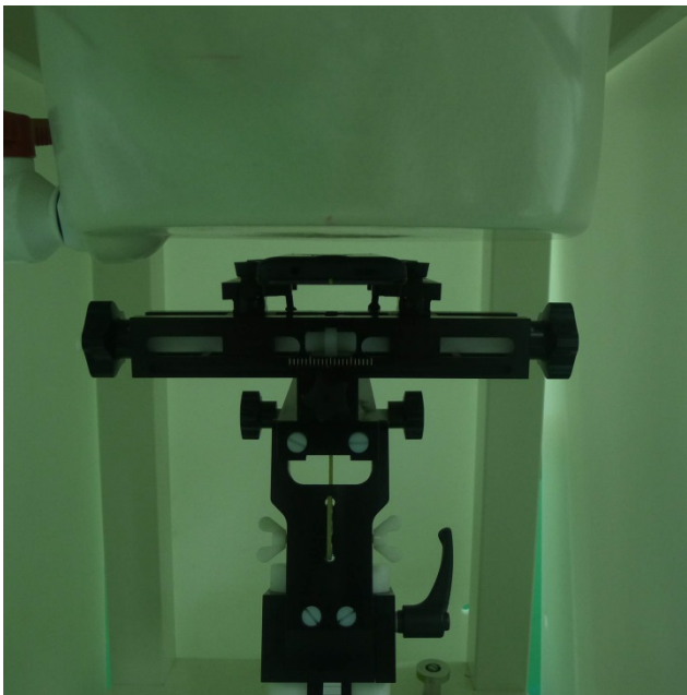
Back of the DUT with Phantom 1 cm Gap
