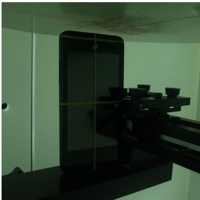
Top Side of the DUT with Phantom 1 cm Gap
