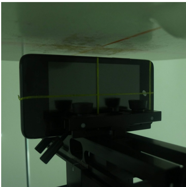
Left Side, Test Separation 1 cm
