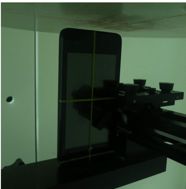
Bottom Side, Test Separation 1 cm
