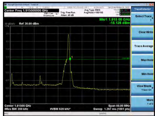
DC_66A_n25A 16QAM 20MHz CH-High 100%RB
