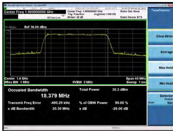
DC_12A_n2A 16QAM 20MHz CH-High
