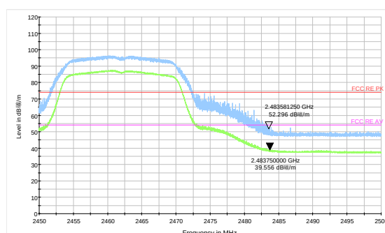
802.11g-Channel 11 Peak+ Average
