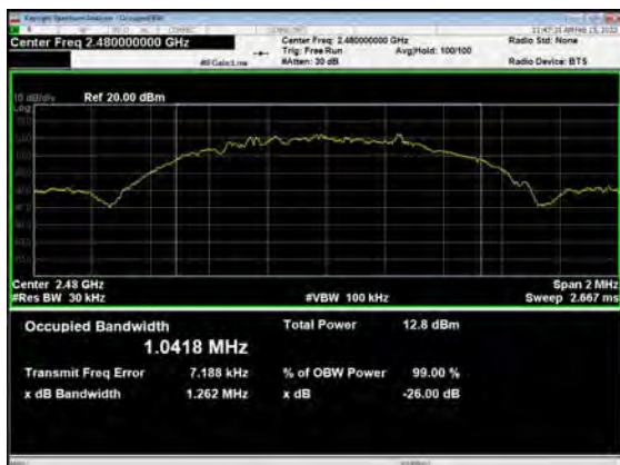
Bluetooth LE (1M) Carrier frequency (MHz): 2480
