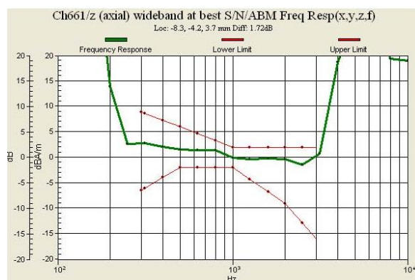
Fig 7.2 GSM1900 Ch661
