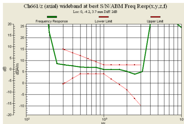
Fig 7.5 GSM1900 Ch661
