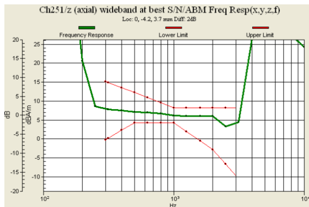
Fig 7.3 GSM850 Ch251
