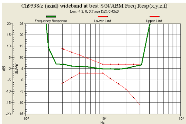
Fig. 7.9 WCDMA Band II Ch9538
