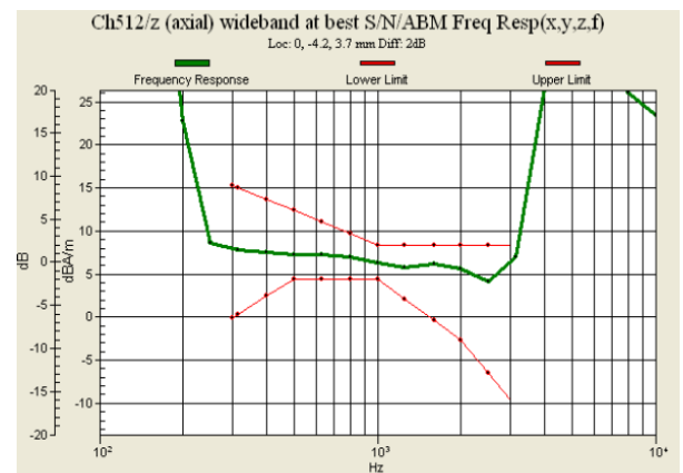
Fig 7.4 GSM1900 Ch512
