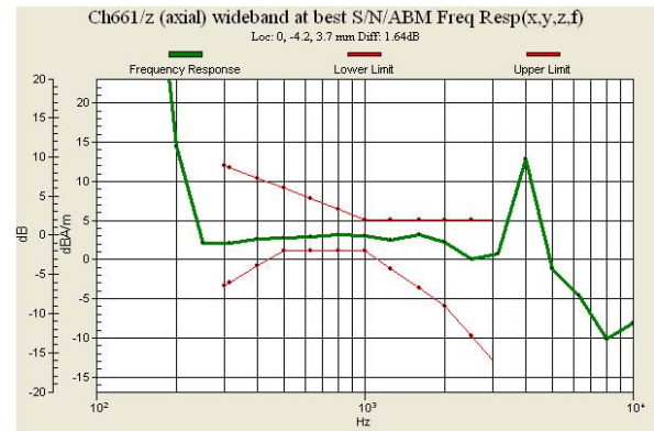
Fig 7.2 GSM1900 Ch661
