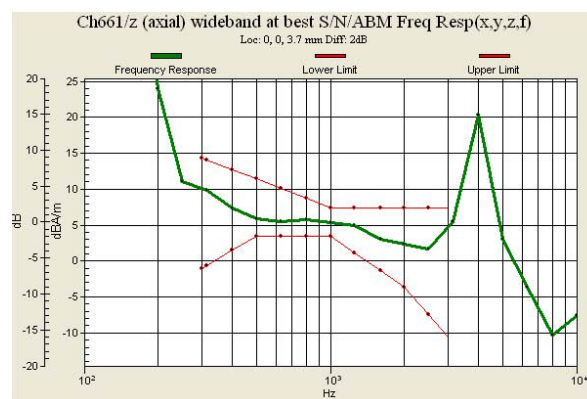
Fig 7.2 GSM1900 Ch661
