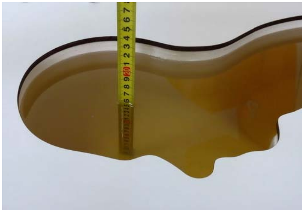
Picture 6: Liquid depth in the head Phantom (835MHz, 15.3cm depth)
