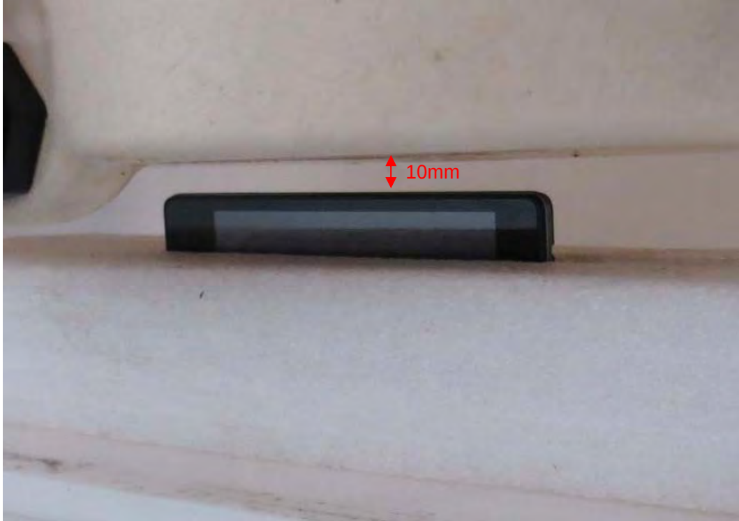
Picture 20: Left Side, the distance from handset to the bottom of the Phantom is 10mm Z815 (RXC1512-0230SAR01R1)
