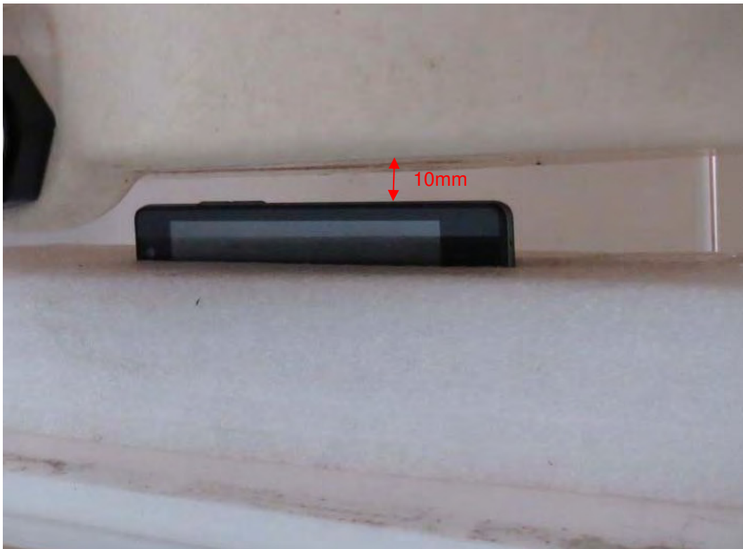
Picture 21: Right Side, the distance from handset to the bottom of the Phantom is 10mm Z815 (RXC1512-0230SAR01R1)
