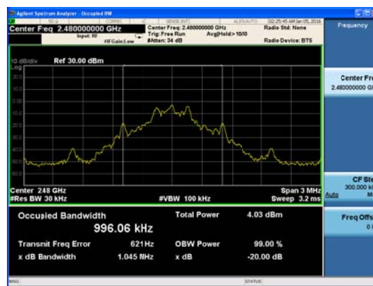
DH5 Channel 78
