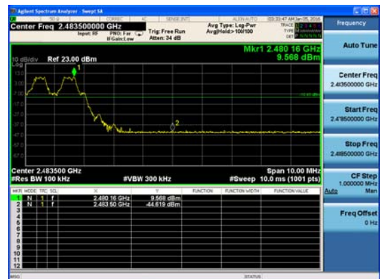
2DH5, Channel 78
