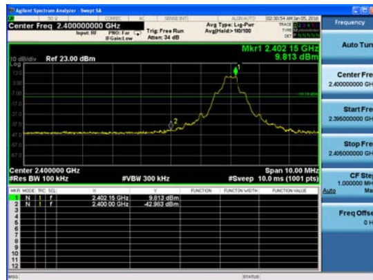
2DH5, Channel 0
