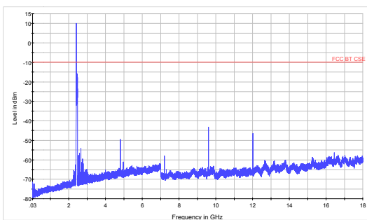
GFSK-CH39 30MHz~18GHz
