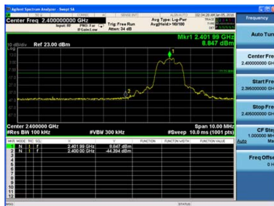
3DH5, Channel 0
