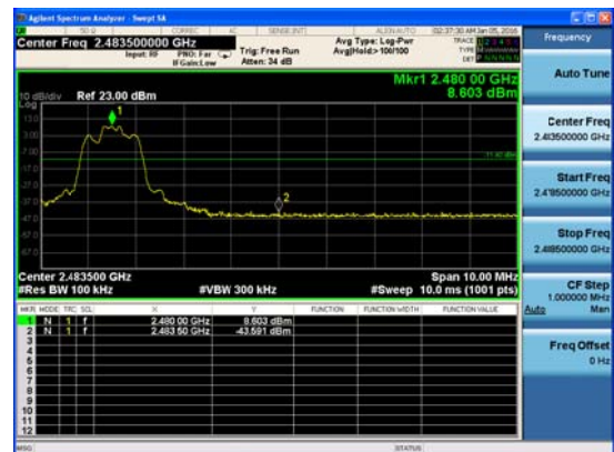
3DH5, Channel 78
