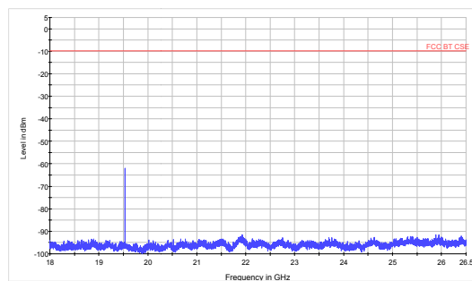
GFSK-CH39 18GHz~26.5GHz
