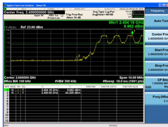
2DH5, Channel 0
