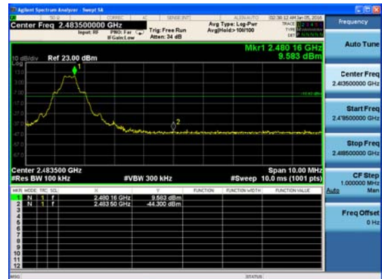
2DH5, Channel 78
