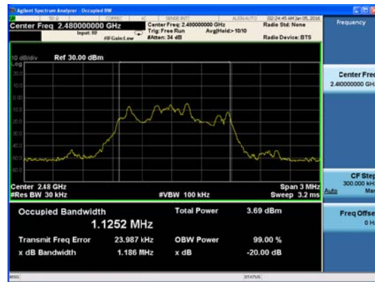
3DH5 Channel 78
