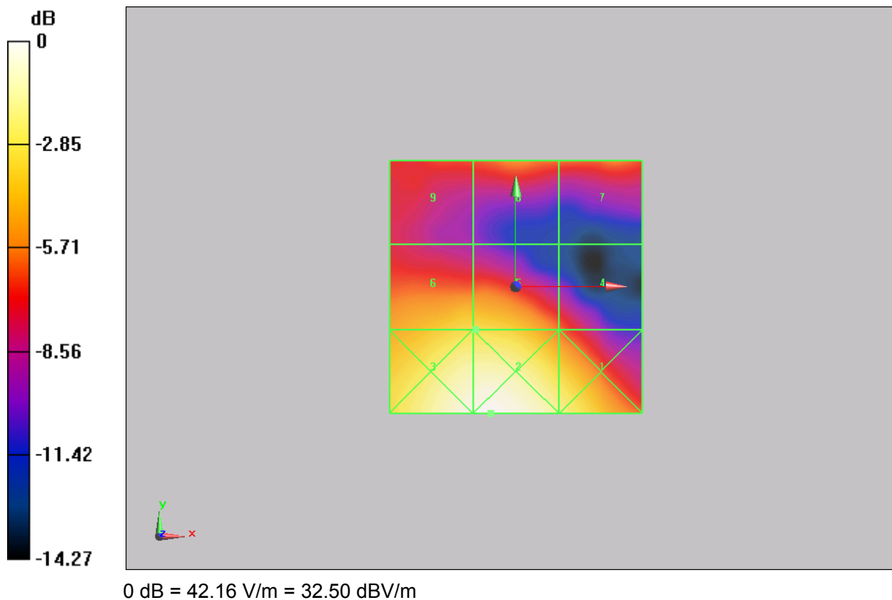
Figure 13 HAC RF E-Field GSM 1900 Channel 512
