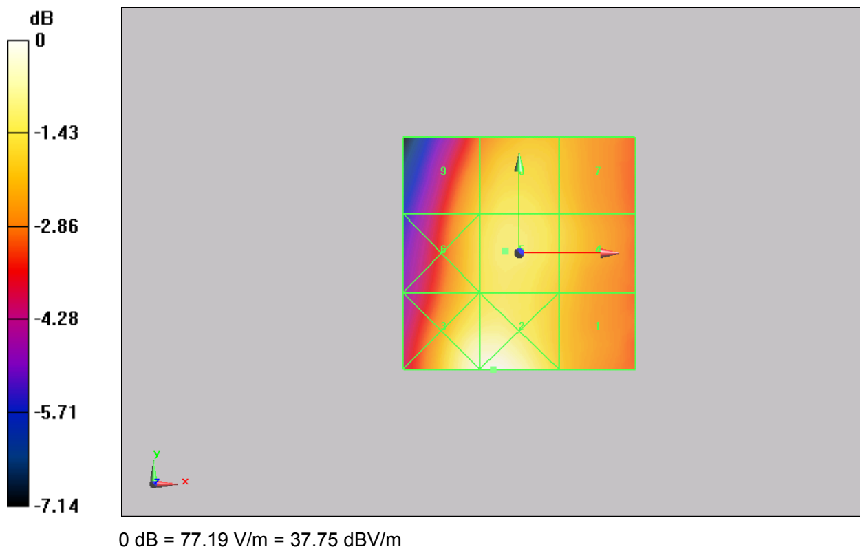
Figure 8 HAC RF E-Field GSM 850 Channel 251
