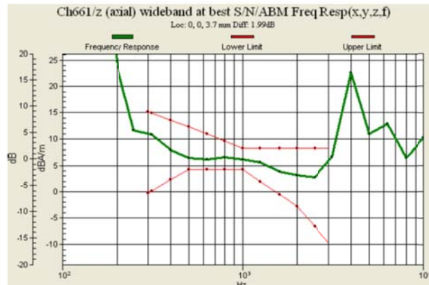
Fig 7.2 GSM1900 Ch661
