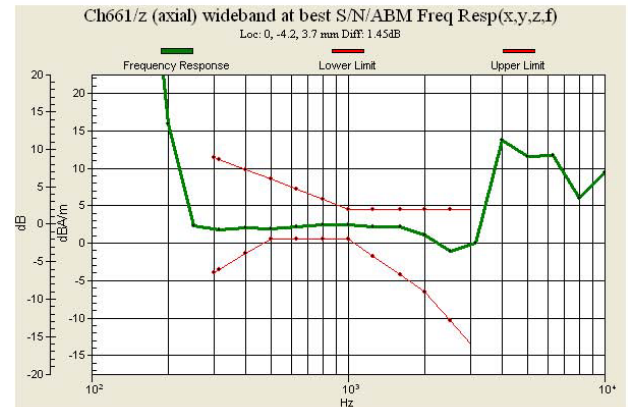
Fig 7.2 GSM1900 Ch661
