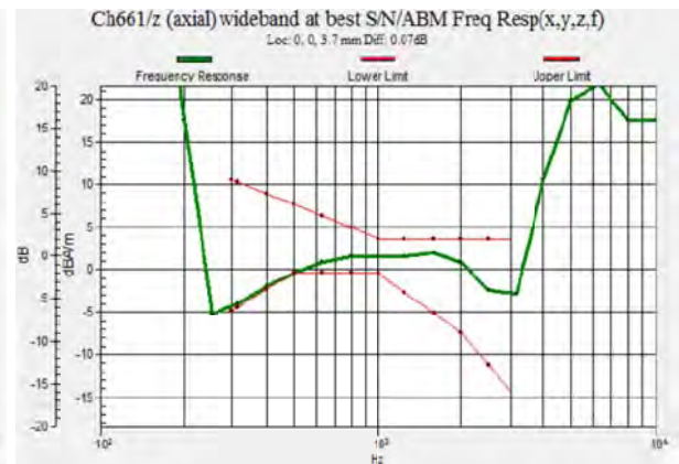
Fig 7.2 GSM1900 Ch661
