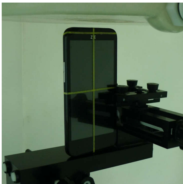
Top Side, Test Separation 10 mm
