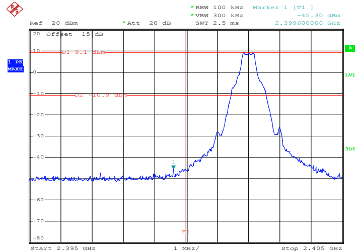
Low Band Edge Plot on Channel 00
