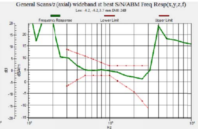
Fig 7.2 GSM1900 Ch661
