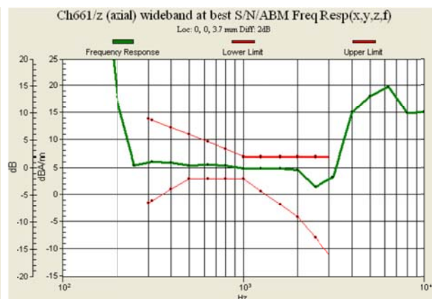
Fig 7.2 GSM1900 Ch661
