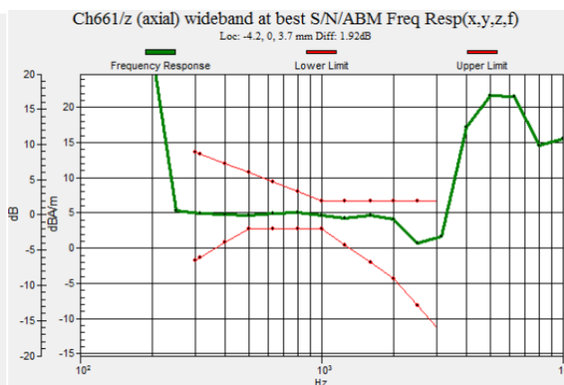
Fig 7.2 GSM1900 Ch661
