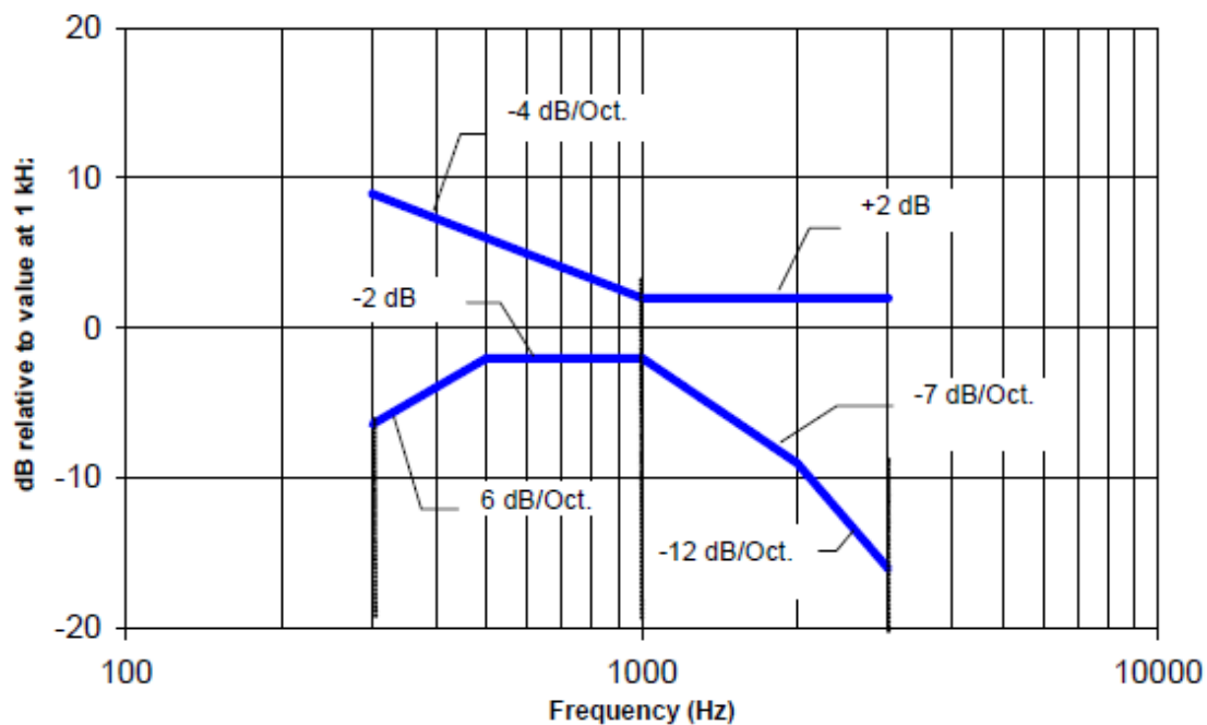
Fig. 4.2 Magnetic field frequency response for WDs with a field that exceeds -15 \text{ dB(A/m)} at 1 kHz
