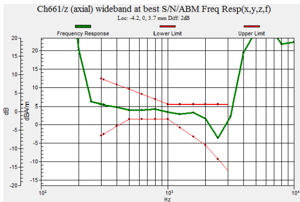
Fig 7.2 GSM1900 Ch661
