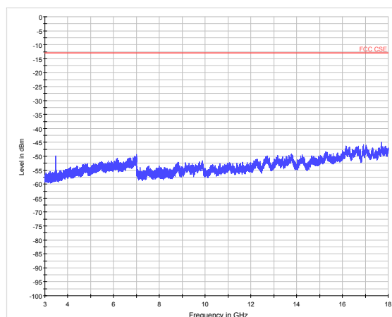
NB-IOT Band 4 15KHz CH-High 3GHz~18GHz
