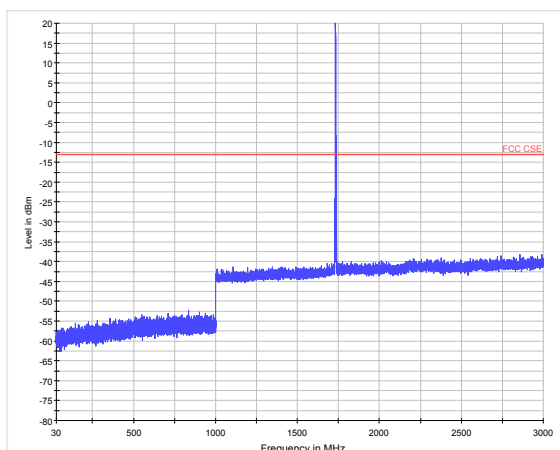
NB-IOT Band 4 15KHz CH-High 30MHz~3GHz
