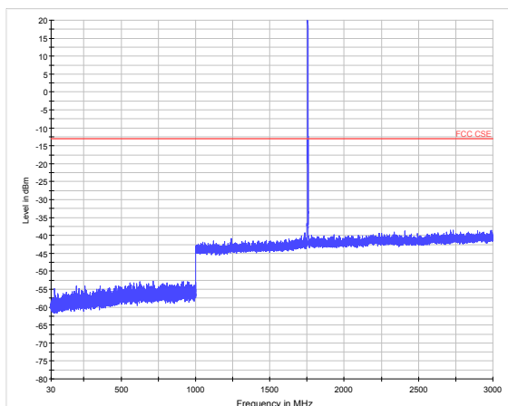
NB-IOT Band 4 15KHz CH-High 30MHz~3GHz
