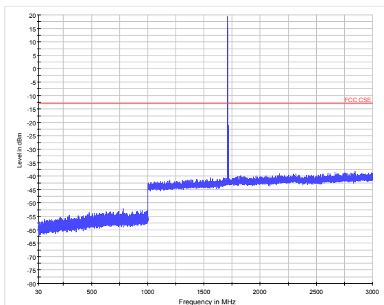
NB-IOT Band 4 15KHz CH-Middle 30MHz~3GHz
