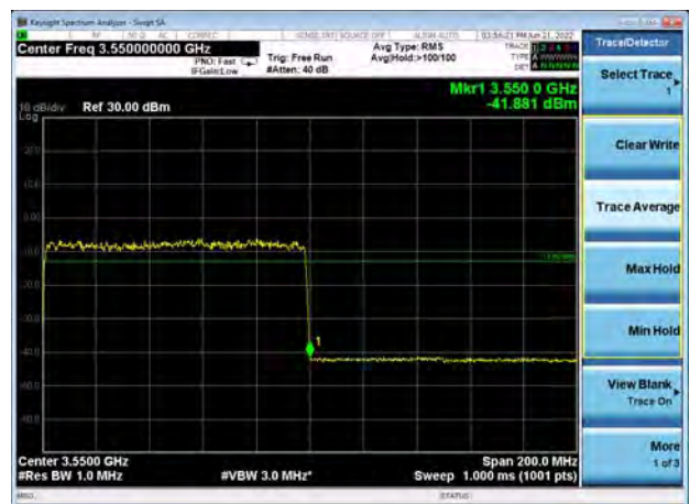
NR n78 Subset 1 25A6QAM 100MHz CH-High 1RB
