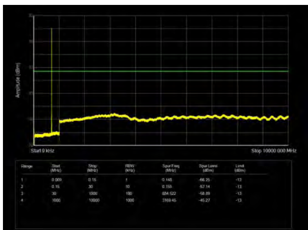
LTE Band 12 1.4MHz CH- Middle 9kHz ~10GHz
