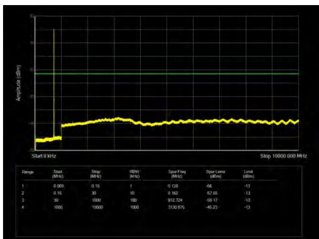
LTE Band 12 1.4MHz CH-High 9kHz ~10GHz
