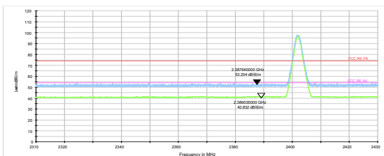
Bluetooth LE Channel 0 Peak+ Average
