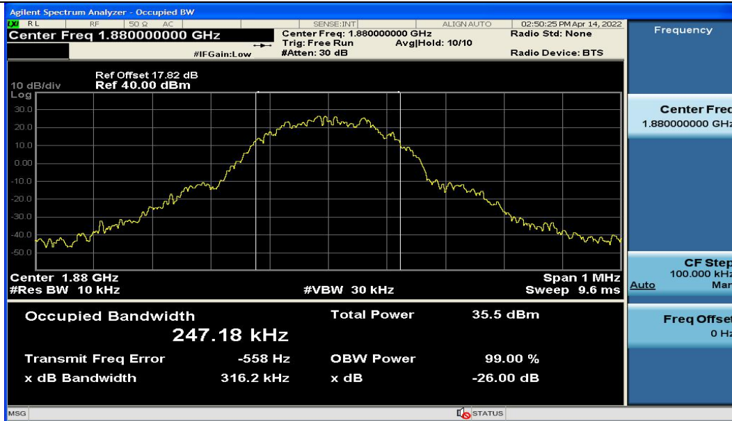
Channel 661
